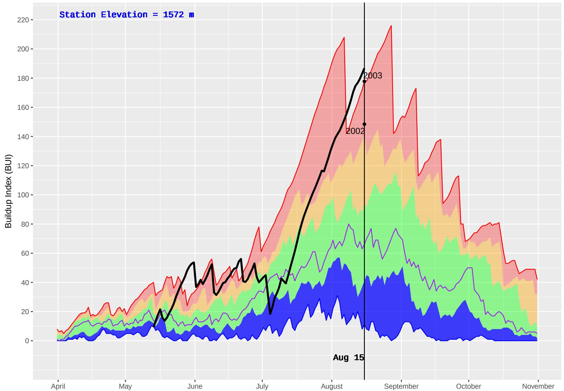
NEGRO CREEK (789) : Historical (2001–2016) and Current (2018) Daily Buildup Index (BUI)
