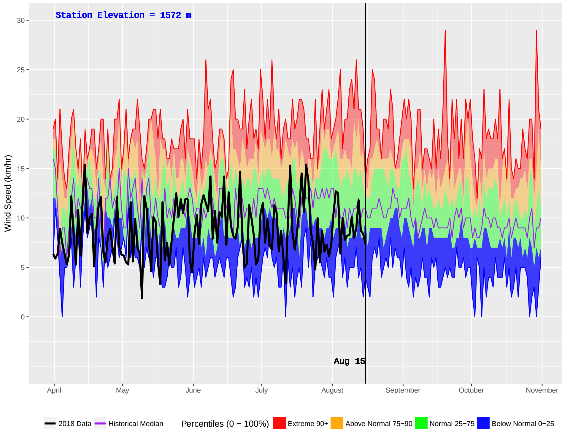
NEGRO CREEK (789) : Historical (2001–2016) and Current (2018) Daily Wind Speed
