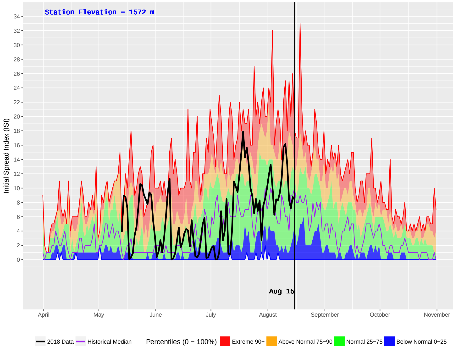
NEGRO CREEK (789) : Historical (2001–2016) and Current (2018) Daily Initial Spread Index (ISI)
