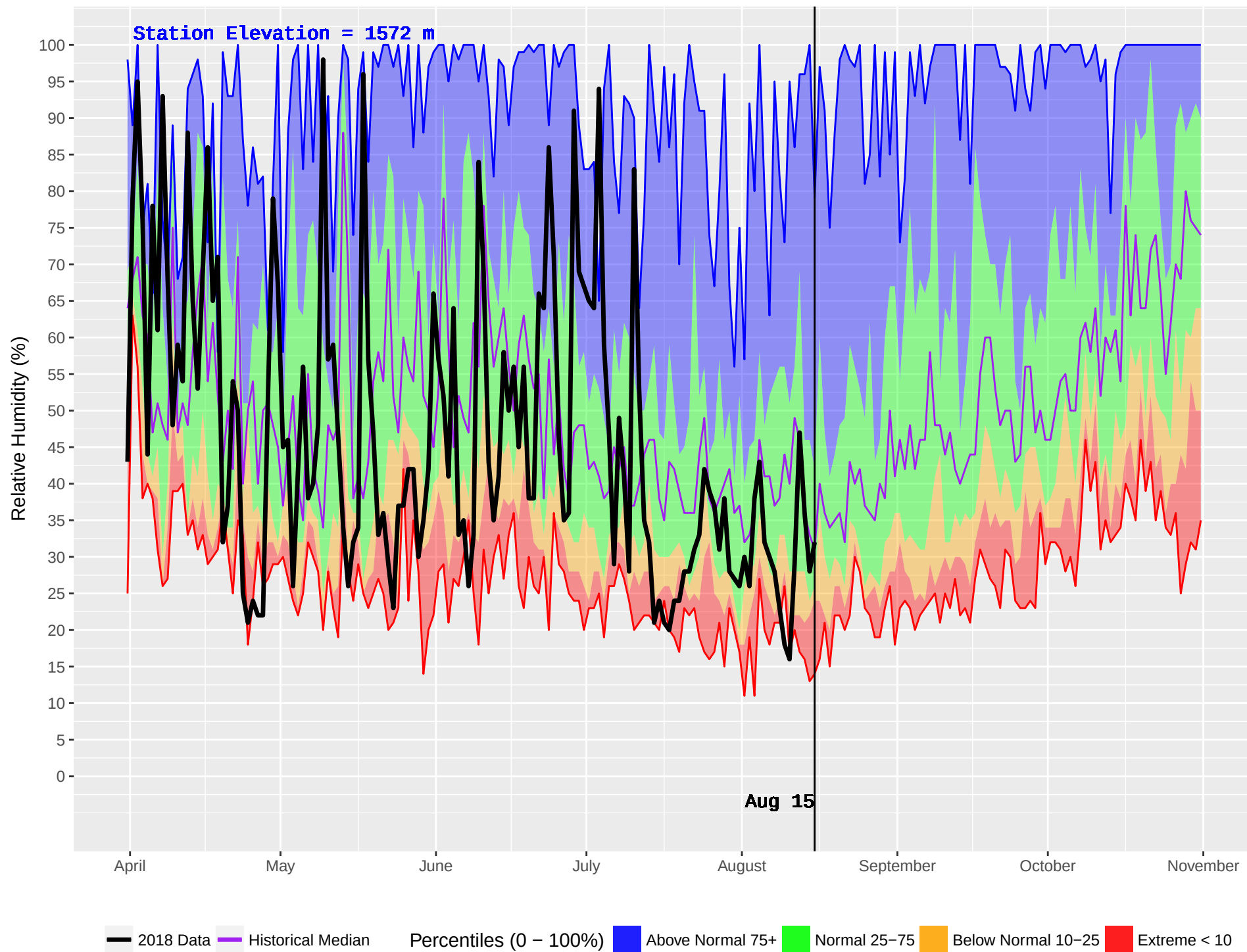
NEGRO CREEK (789) : Historical (2001–2016) and Current (2018) Daily Relative Humidity
